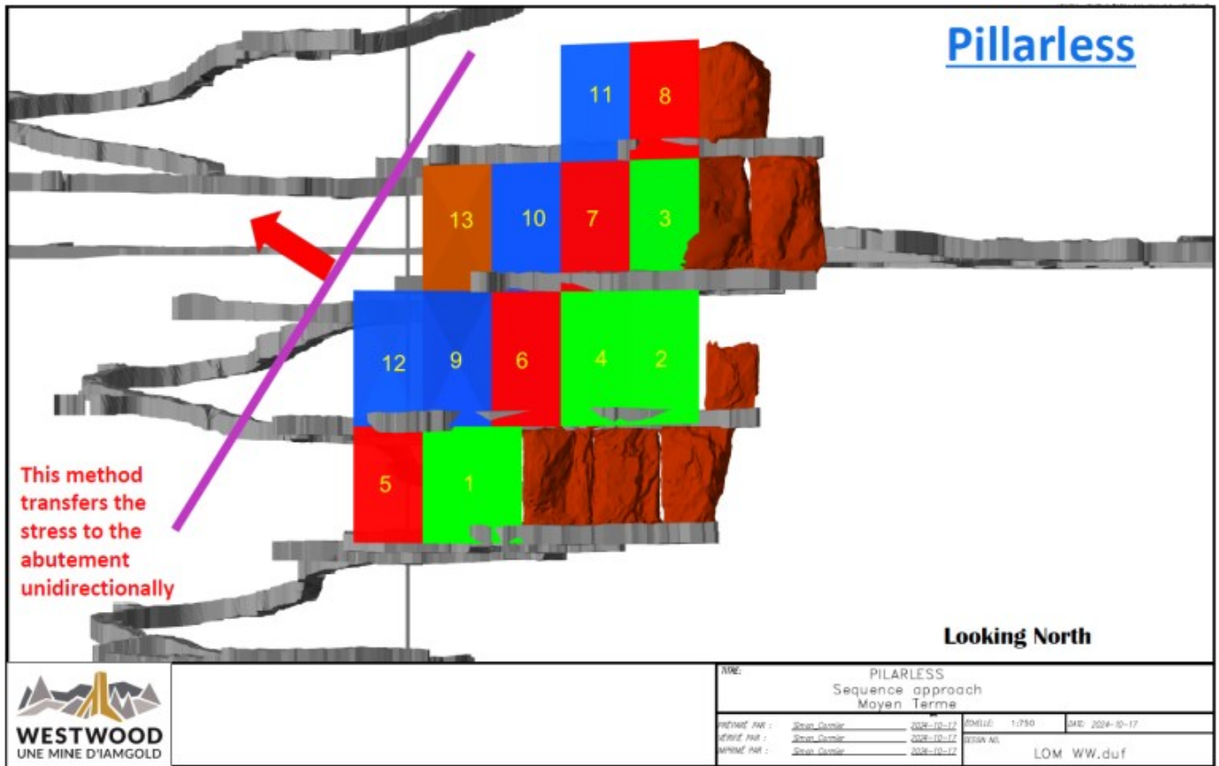
Figure 16-4: Current Mining Method, Westwood
