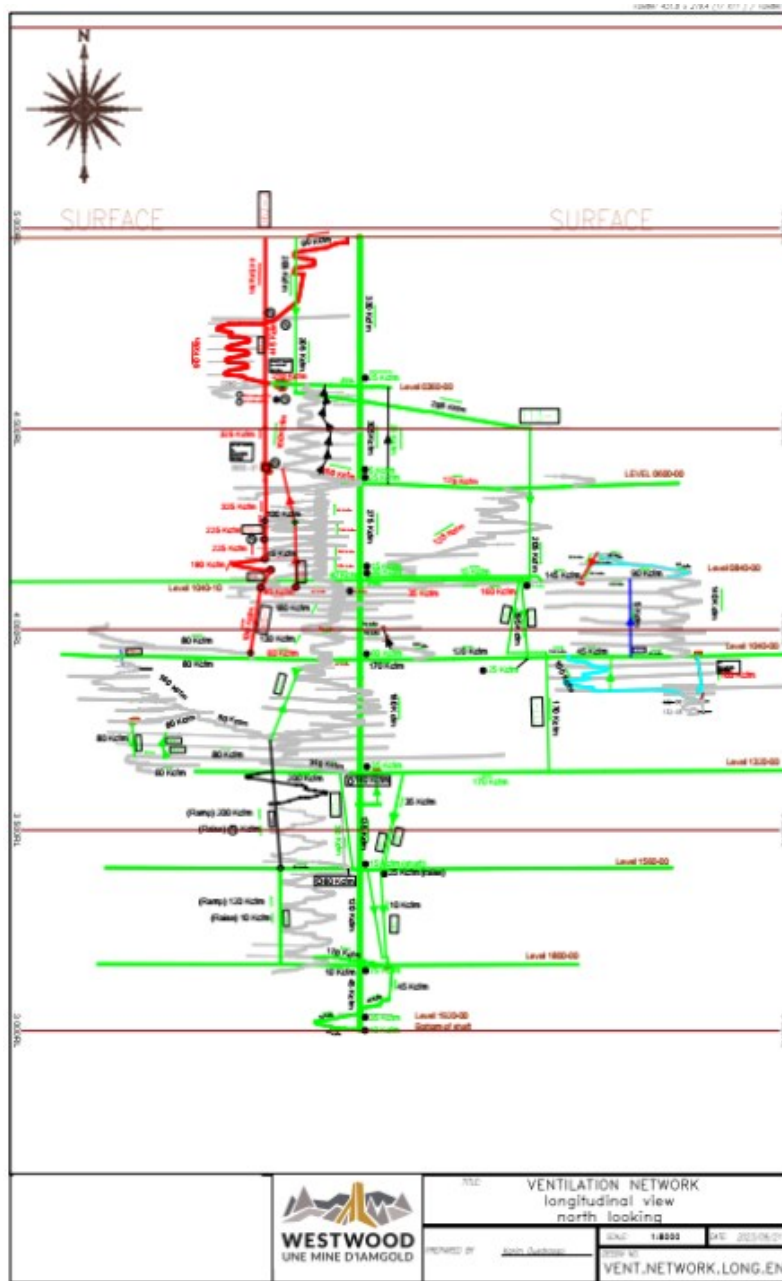
Figure 16-6: Ventilation System Layout Schematic
