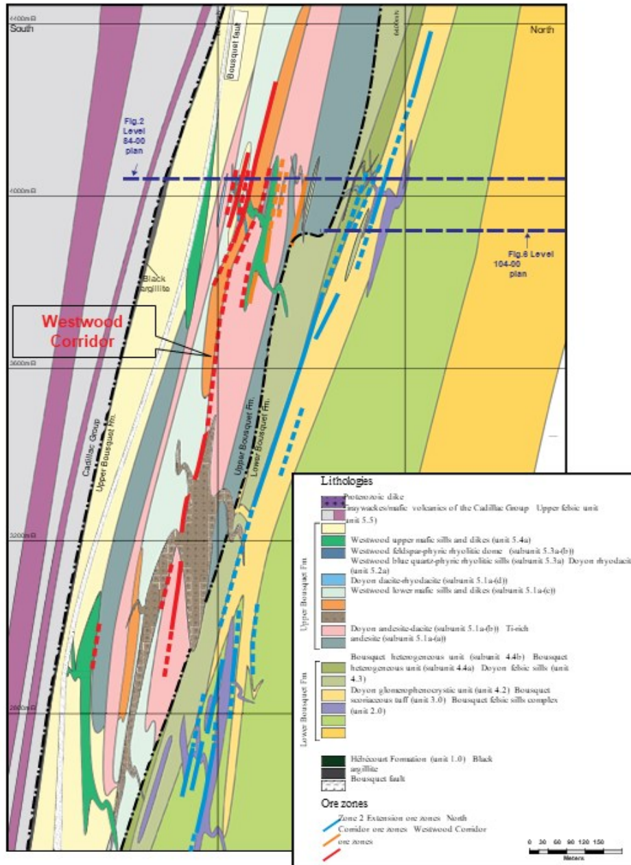
Figure 7-12: Cross-Section Showing Mineralization, Westwood Corridor
