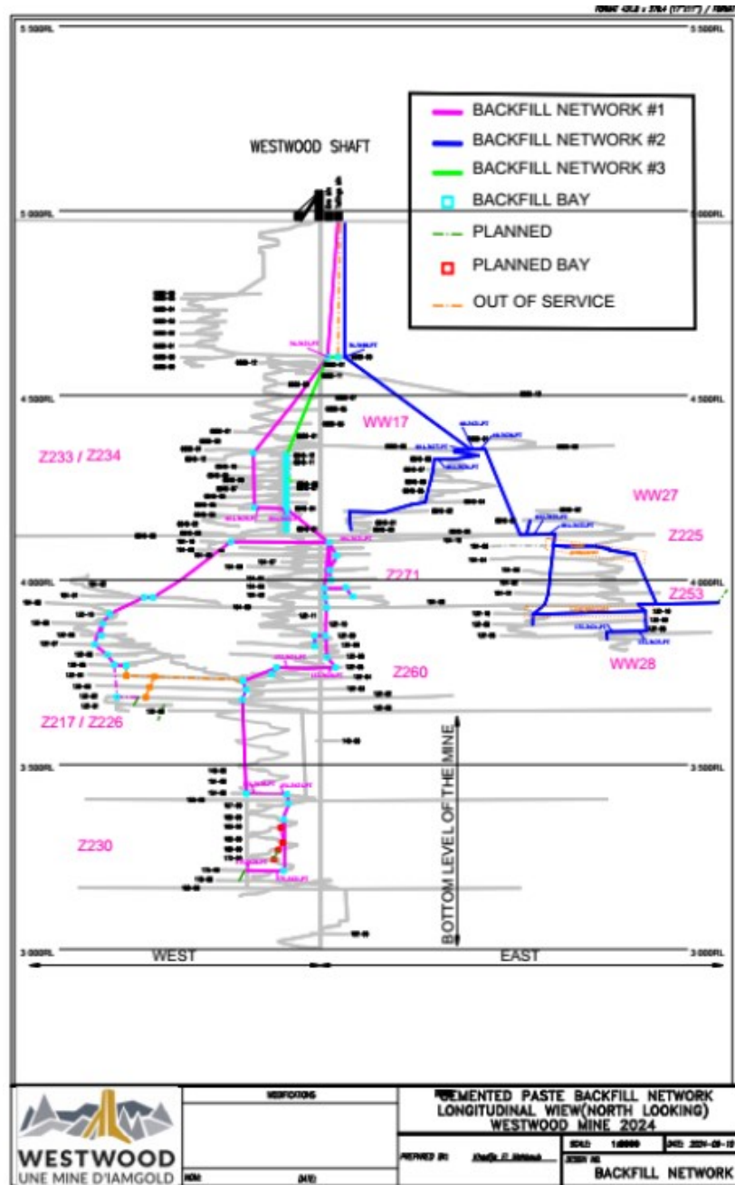
Figure 16-7: Backfill System Layout Schematic
