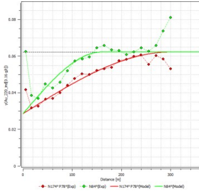
Figure 14-5: Semi-Variogram Of Cut-Off #1 As An Example (WW28A)
