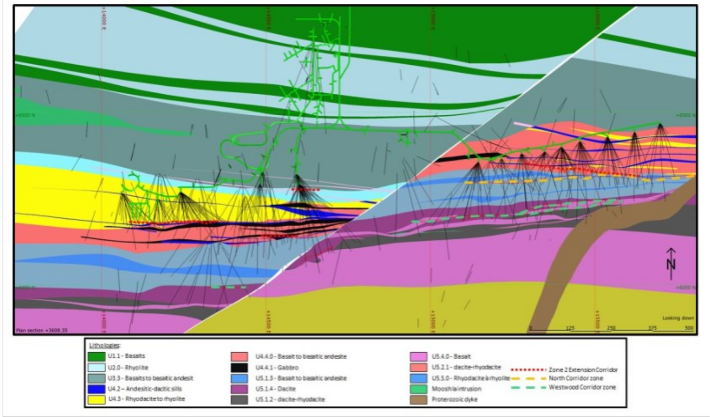
Figure 7-7: Geological Map - Plan View of Level 132-00
