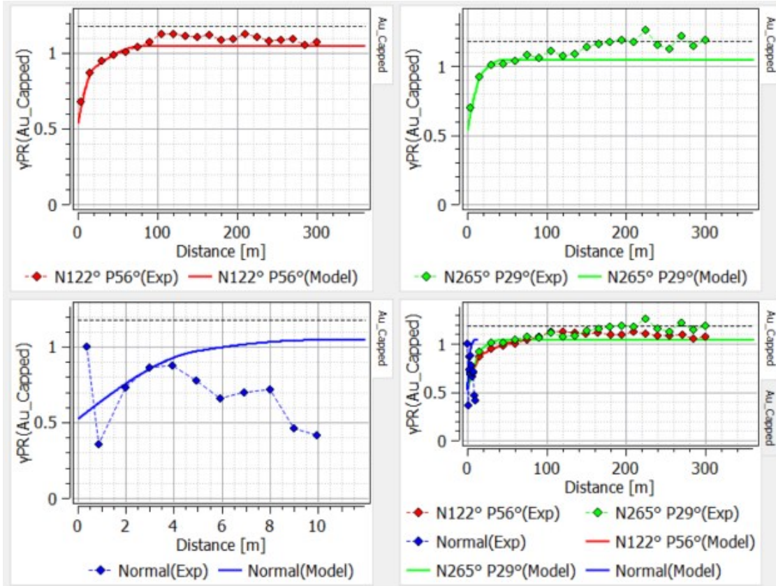
Figure 14-3: Variography Study for Group F
