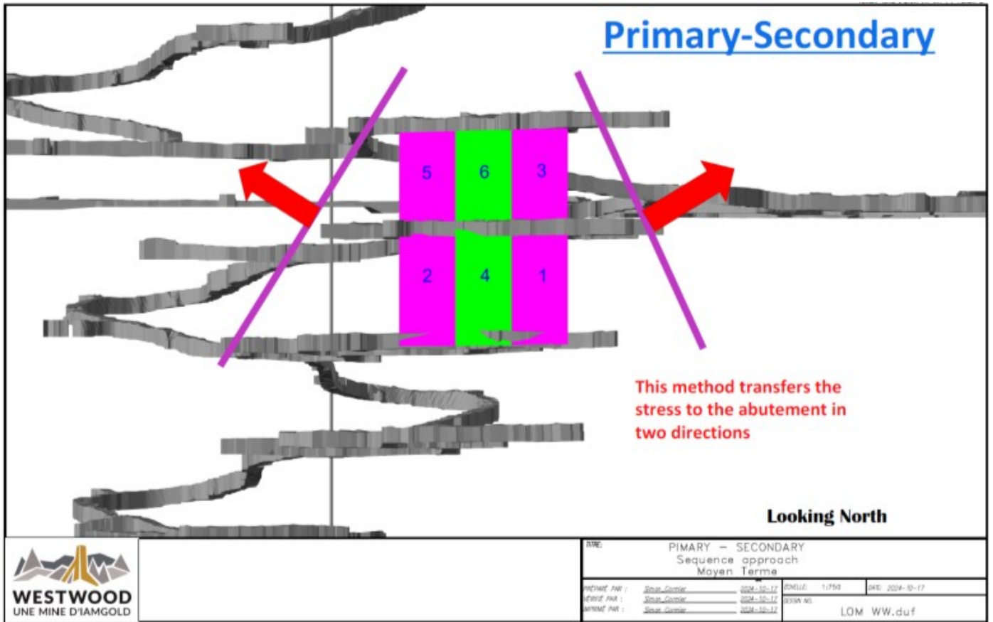
Figure 16-3: Former Mining Method, Westwood
