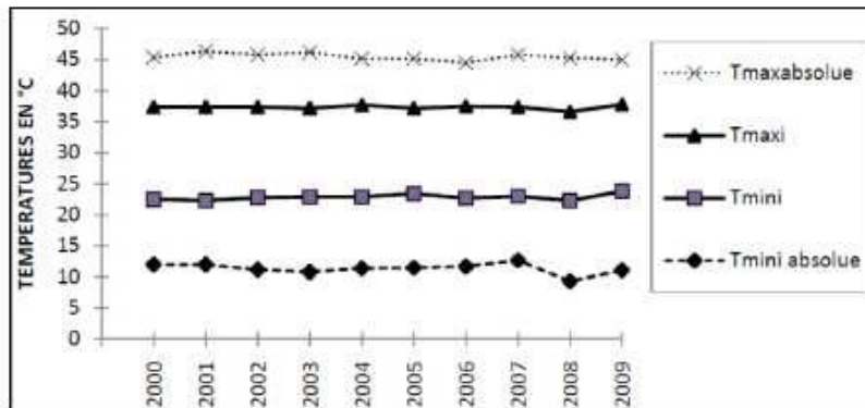
Figure 5.3: Temperature Evolution at Dori (2000-2009) (Yameogo 2011)
