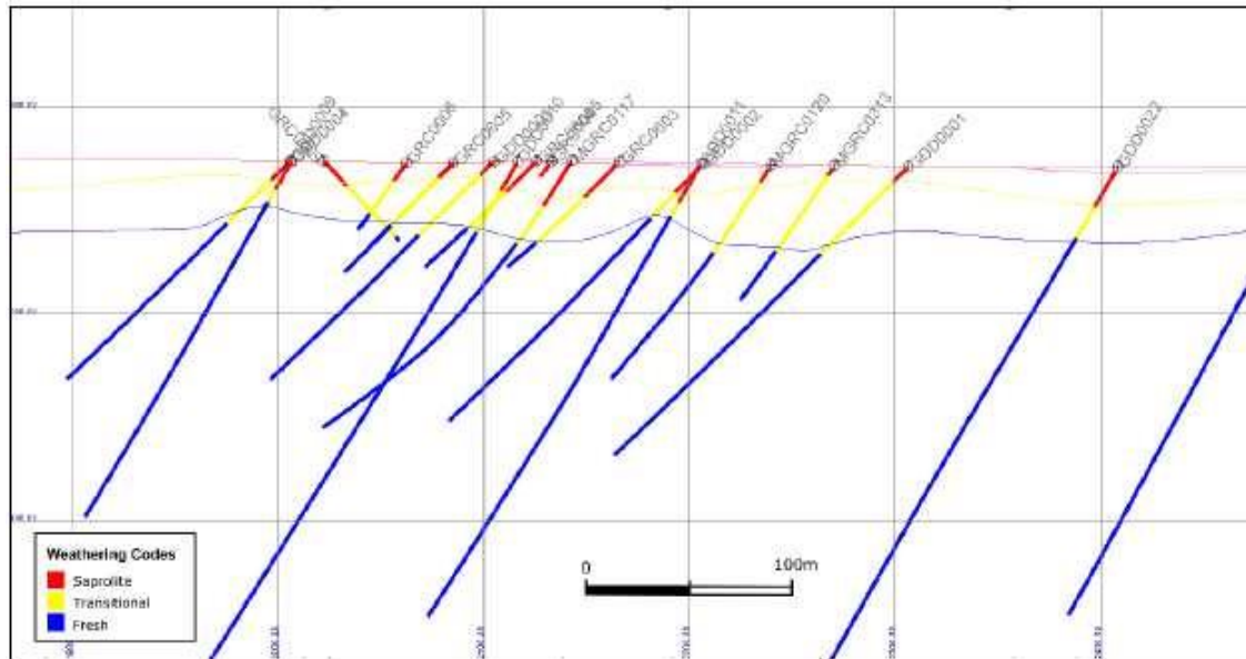
Figure 14.2: Weathering Profile Model - Section 18100 Looking NE
