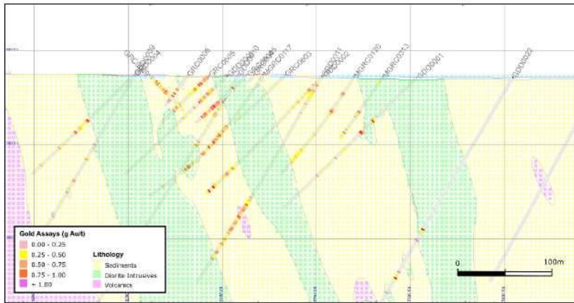
Figure 14.3: Lithology Interpretation and Gold Assays – Section 18100
