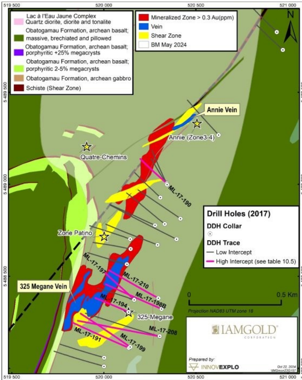
Figure 10.5 - Holes drilled by IAMGOLD on the Monster Lake Property in 2017
