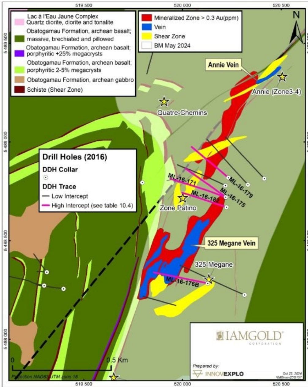
Figure 10.4 - Holes drilled by IAMGOLD on the Monster Lake Property in 2016
