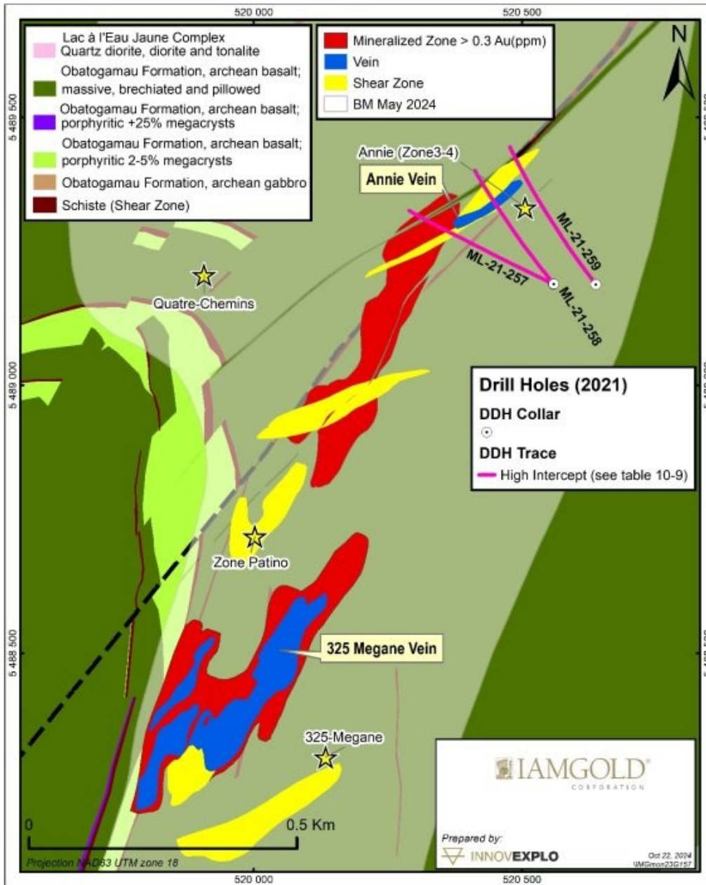
Figure 10.9 - Holes drilled by IAMGOLD on the Monster Lake Property in 2021
