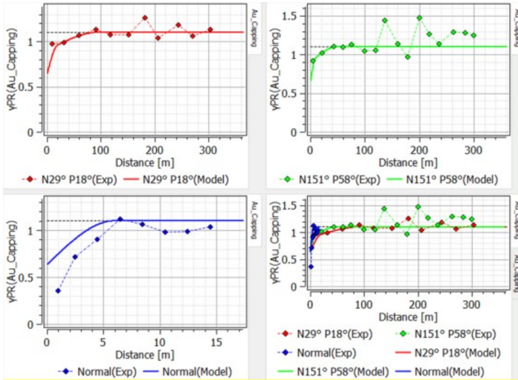
Figure 14.4 - Example of the variography study for Zone 1
