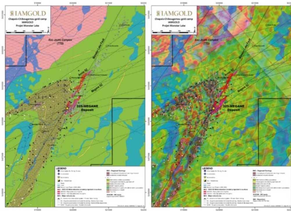
Figure 7.9 - Close-ups of the Monster Lake property, key gold showings, zones and structures
