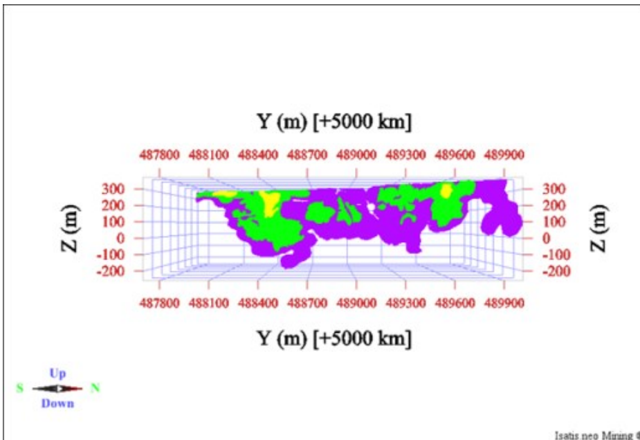
Figure 14.11 - Classified Mineral Resources Within the Constraining Volumes for the Monster Lake Gold Project (Looking West) (4 = Indicated, 5 = Inferred, 6 = Exploration Potential)
