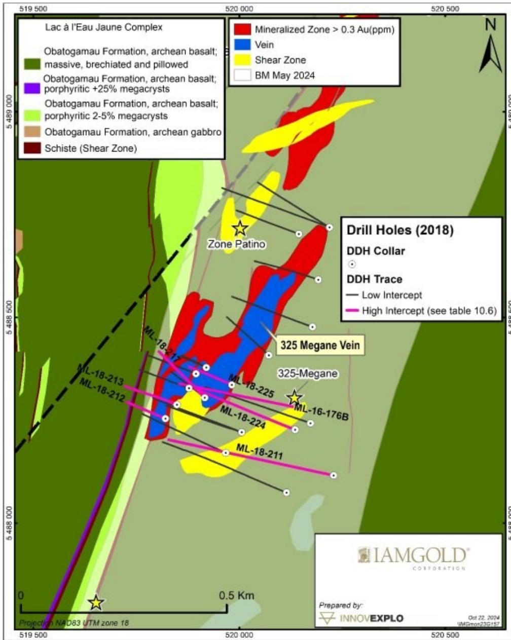
Figure 10.6 - Holes drilled by IAMGOLD on the Monster Lake Property in 2018
