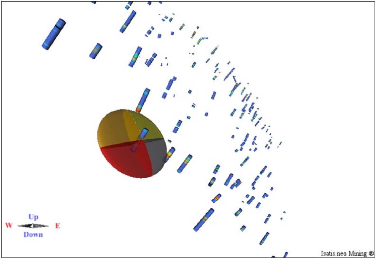
Figure 14.3 - Section Views of the Ellipsoid Radii for Zone 1 (Code 101)
