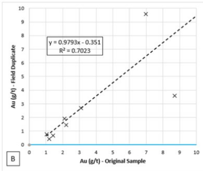
Figure 12.5 - A) Linear graph comparing originals to field duplicates (12 samples) from the resampling program; B) Close-up showing samples under 10 g/t Au
