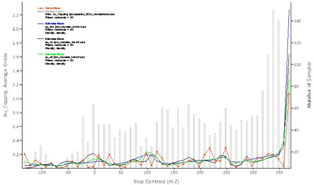
Figure 14.8 - Plot Comparison for Zone Megane (Code 101) of Block Estimates along Vertical Axis/Section
