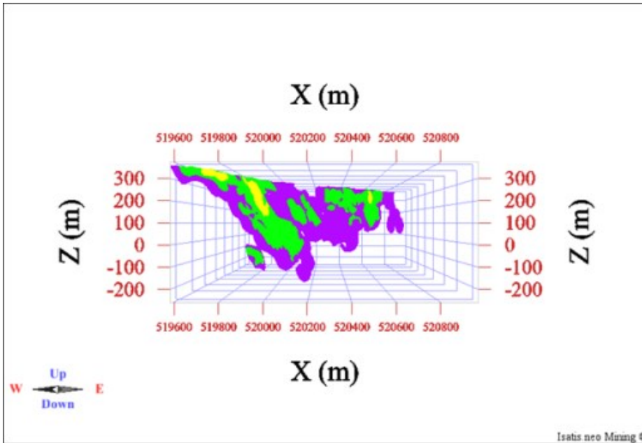
Figure 14.10 - Classified Mineral Resources Within the Constraining Volumes for the Monster Lake Gold Project (Looking North) (4 = Indicated, 5 = Inferred, 6 = Exploration Potential)
