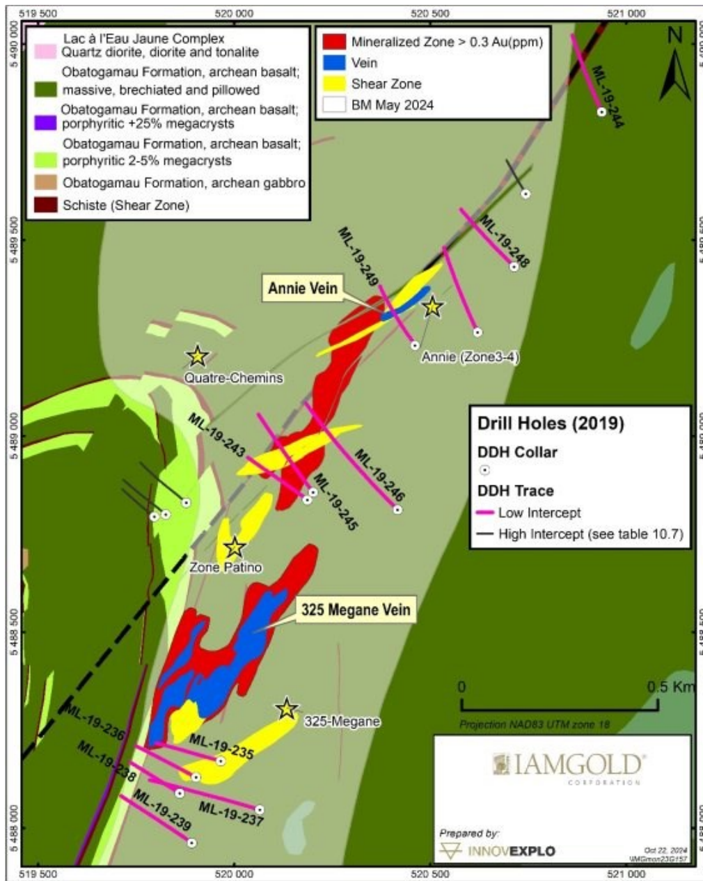
Figure 10.7 - Holes drilled by IAMGOLD on the Monster Lake Property in 2019
