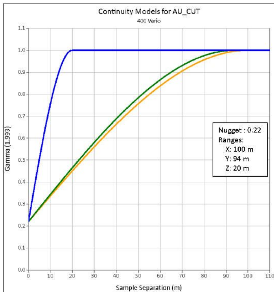
Figure 14.7 – Continuity models for the 325-LG zone (400)
