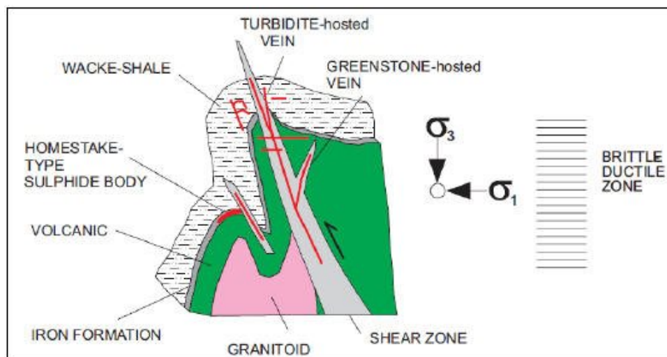
Figure 8.2 – Schematic diagram illustrating the setting of greenstone-hosted quartz-carbonate vein deposits (from Poulsen et al., 2000)
