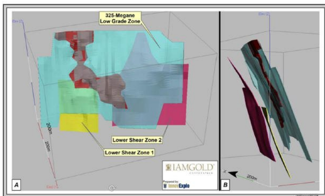
Figure 14.2 – 3D views of the mineralized model for the Monster Lake area: a) pseudo-longitudinal view looking WNW; b) pseudo-cross section view looking NE
