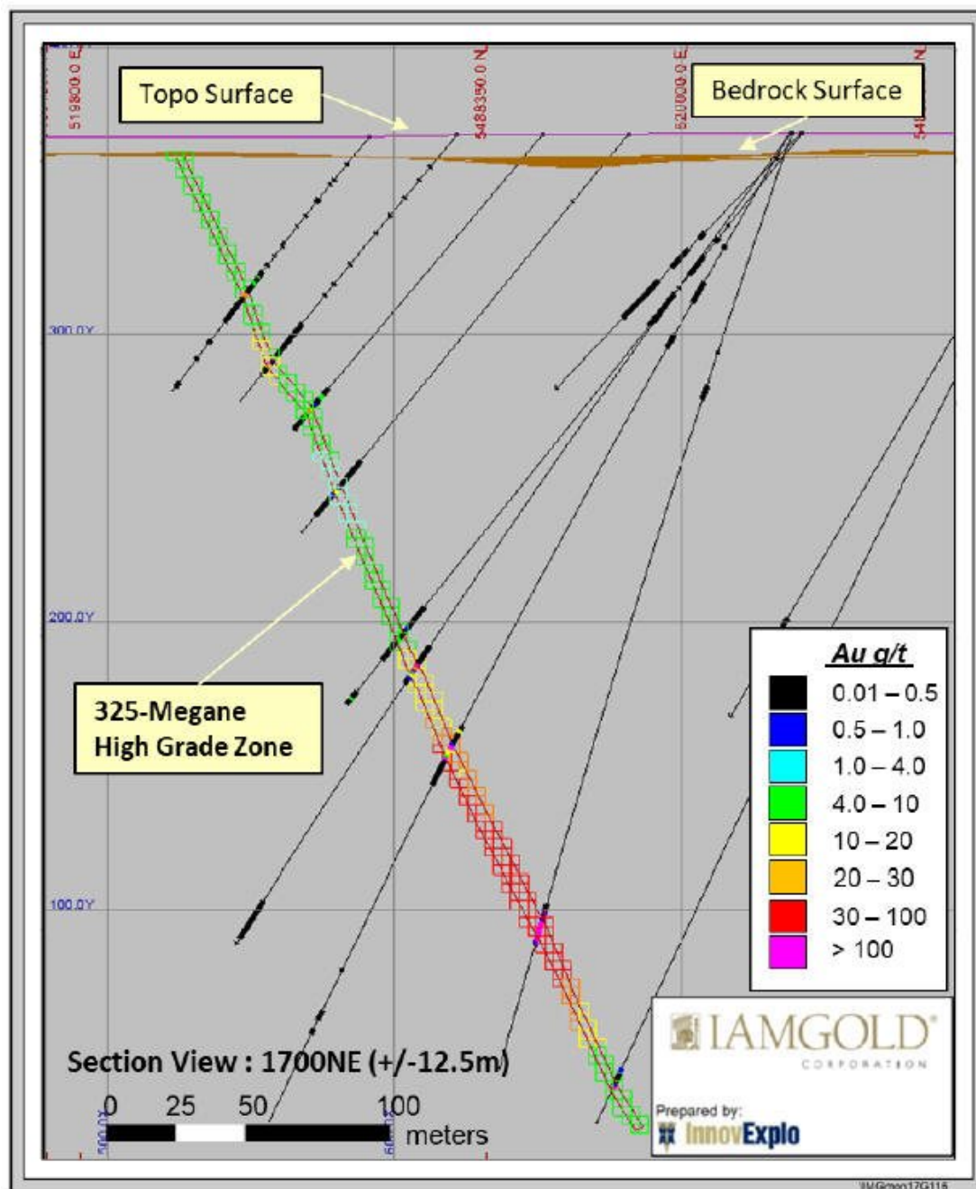
Figure 14.9 – Block model grade for the 325-HG zone, Section 1700NE ( \pm 12.5 m) looking N20
