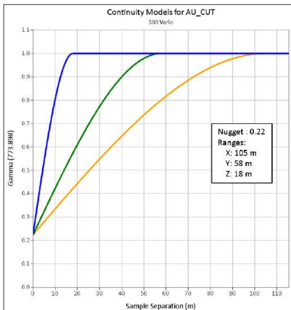
Figure 14.6 – Continuity models for the 325-HG zone (300)
