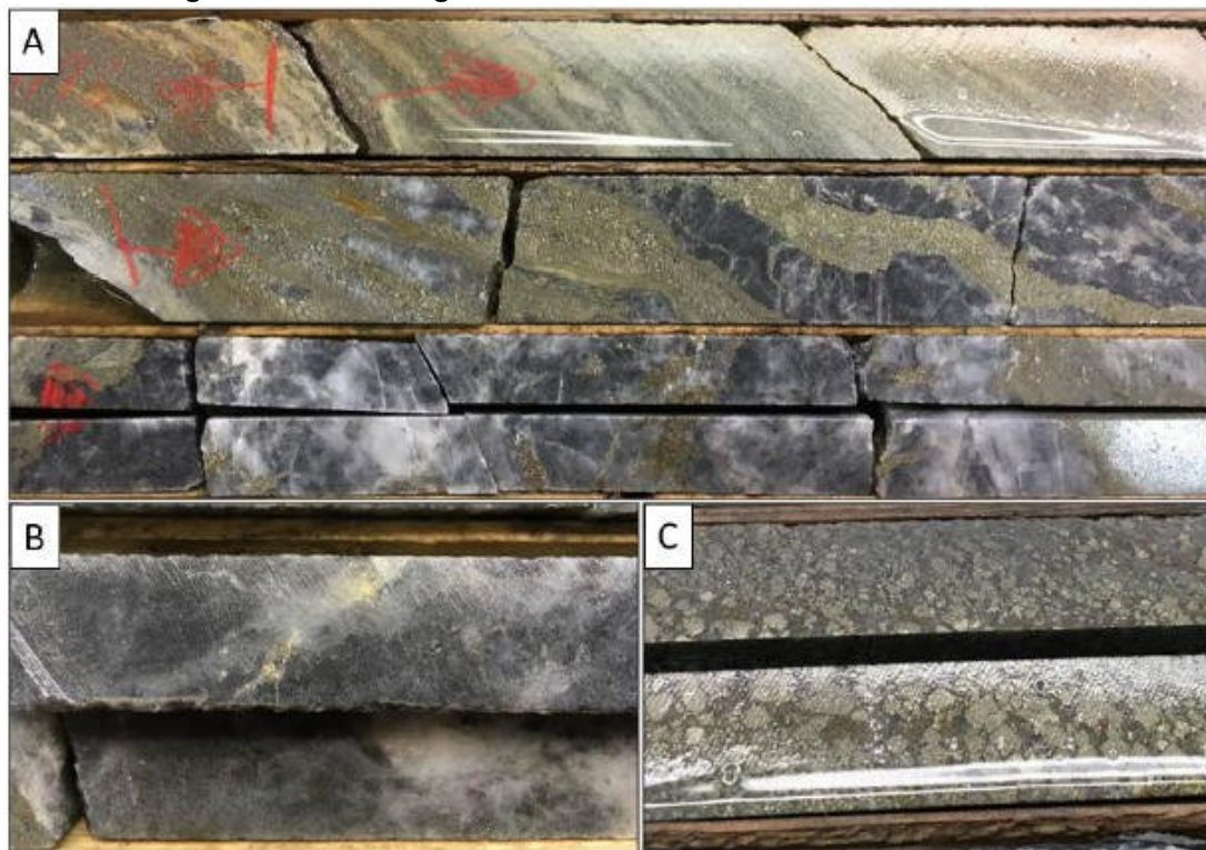
Figure 7.9 – Close-ups of the 325-Megane Zone in hole ML-17-194 : A) Sheared basalt with sericite-ankerite ± fuchsite alteration assemblage (top row), semi-
