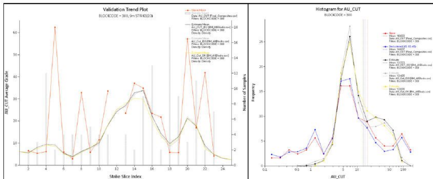
Figure 14.13 – X-direction swath plot and histogram for the 325-HG Zone
