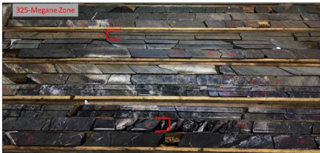
Figure 7.8 – 325-Megane Zone from hole ML-17-194
