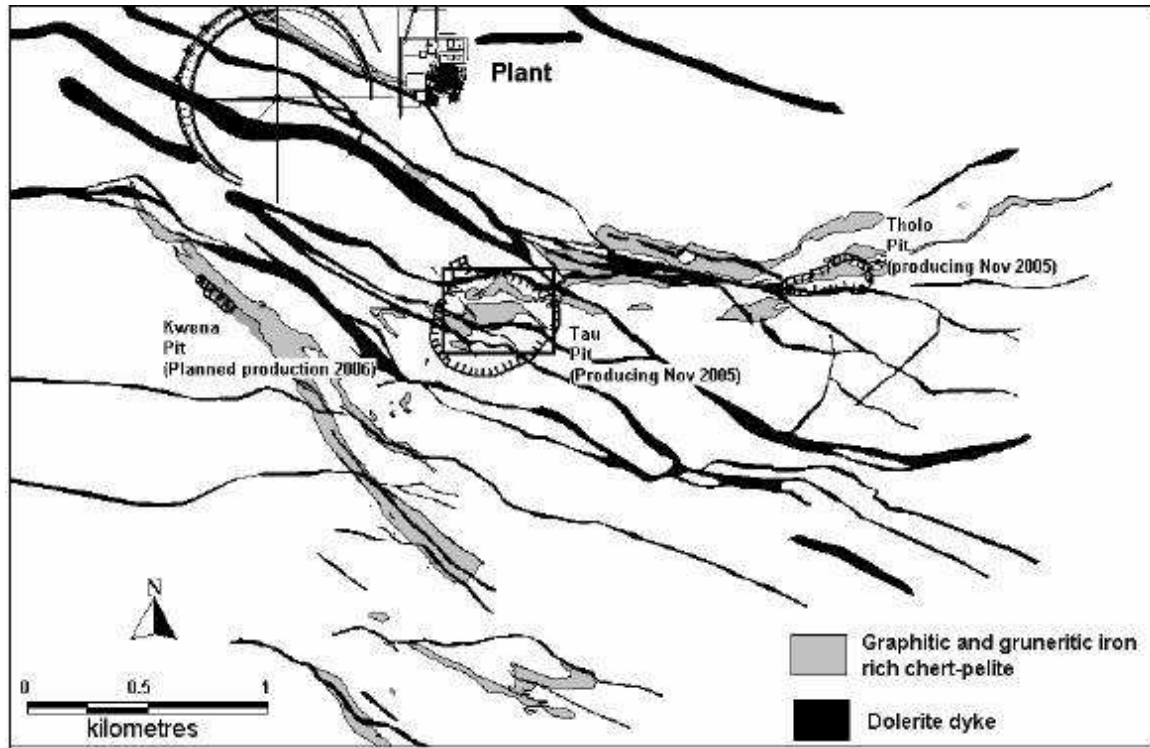
Figure 11.1 Generalized geology of the Mupane region
