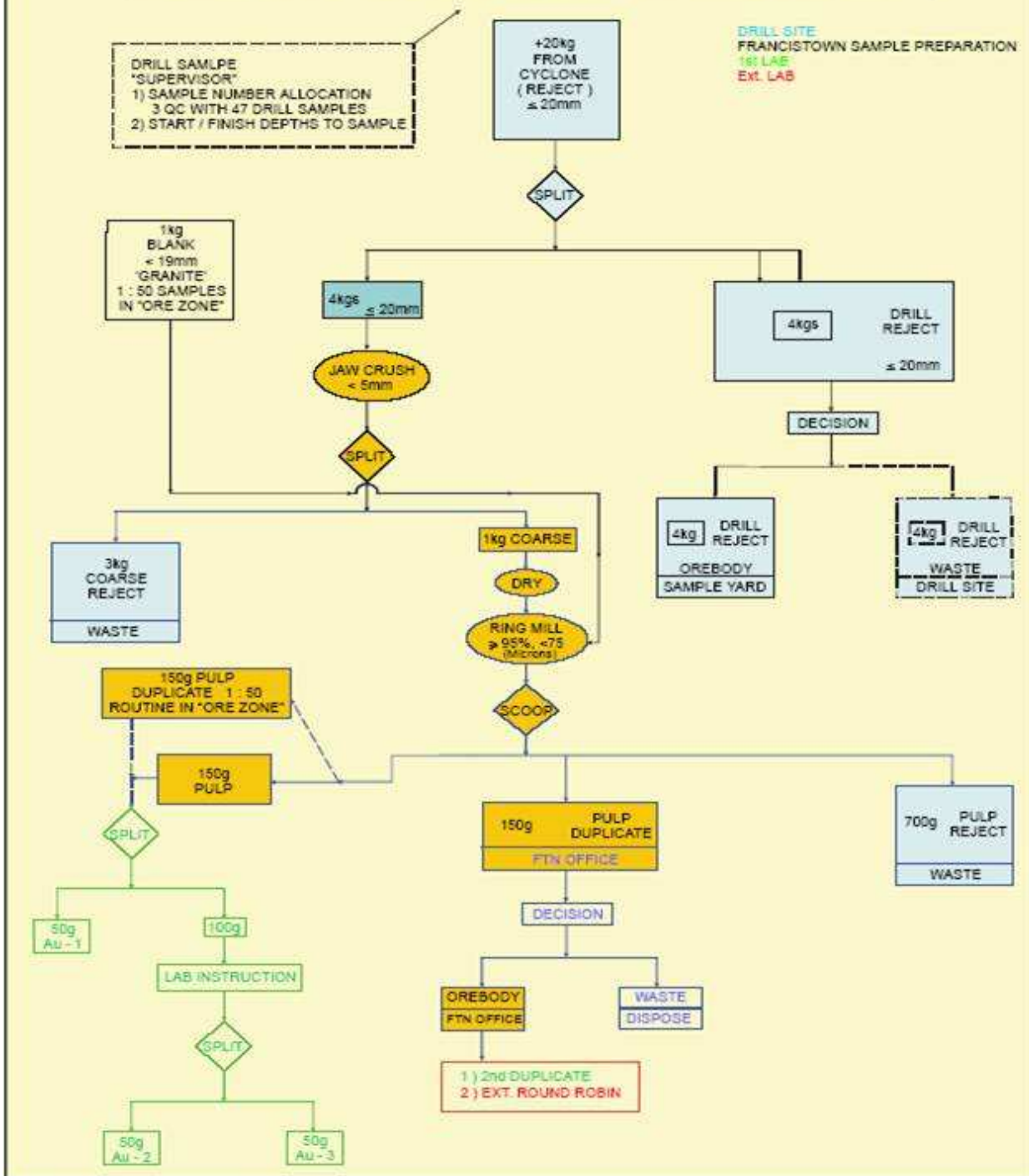
Figure 15.1 Flow sheet for sample preparation at Gallery Gold Botswana
