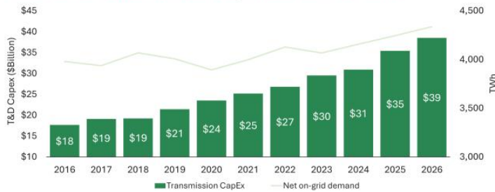
Total Estimated Transmission Capex and Power Demand
